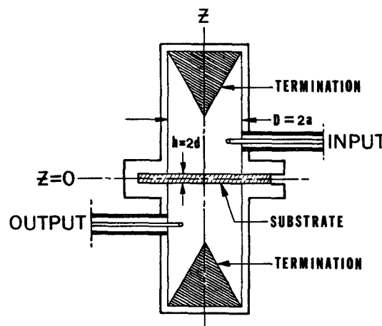
Fig. 1. Schematic cross section of substrate tester.
