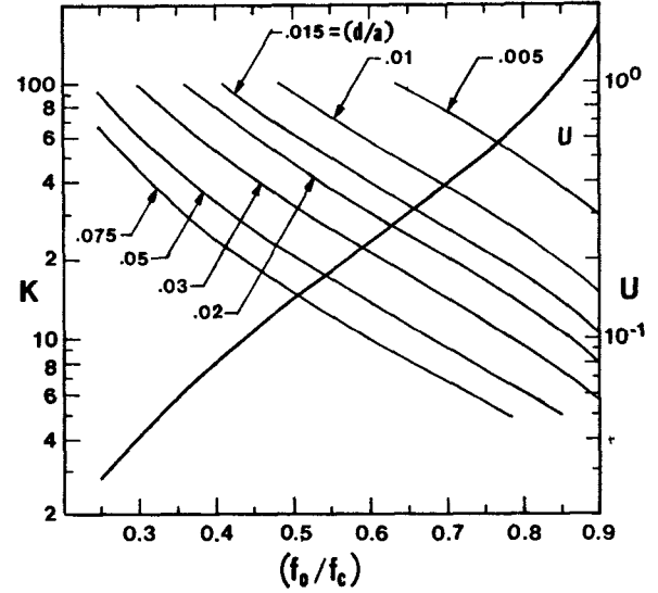
Fig. 2. Curves of K vs. (f_o/f_c) of the TE_{01} mode.
