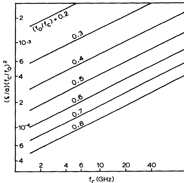
Fig. 3. Plot of (\delta/a)(f_c/f_0)^2 vs. f_c for brass waveguide.
